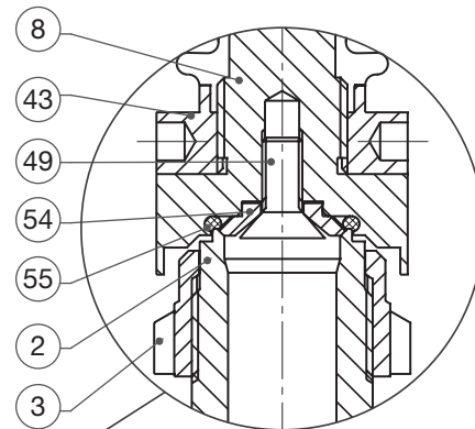
Figure 10a: D - J Orifice
