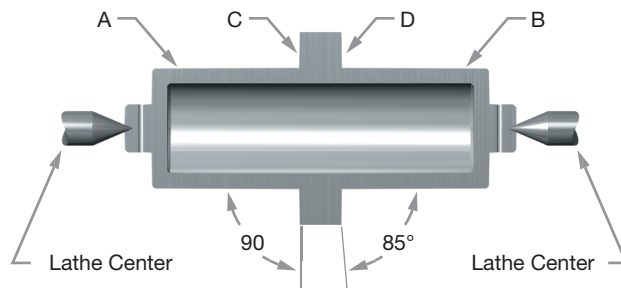
Figure 23: Nozzle Lap in a Lathe
