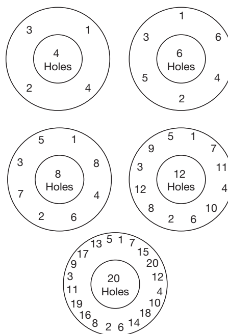
Figure 36: Bolt Tightening Patterns
