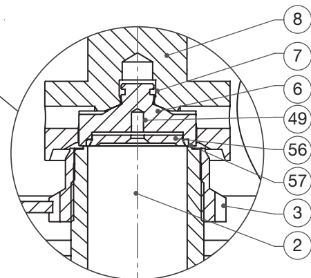
Figure 10c: UM Teflon™ Seal
