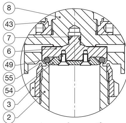
Figure 10b: K-U Orifice
