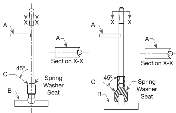
Figure 26: V-Block Support Setup
